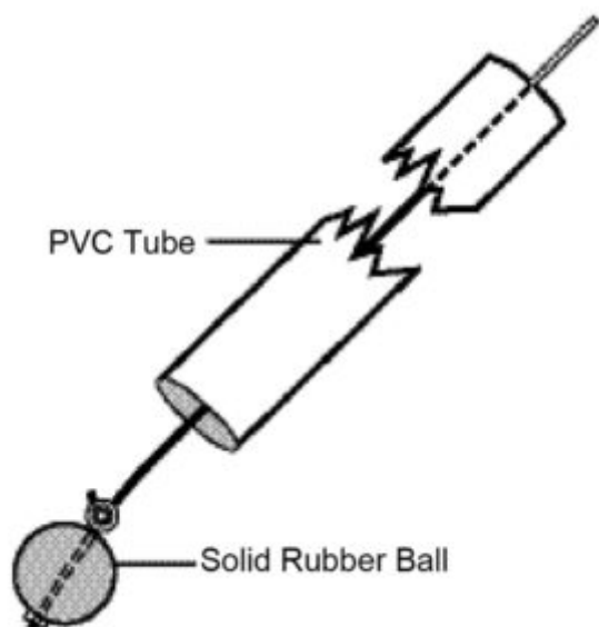
Fig. 1: A simple water column sampler.
