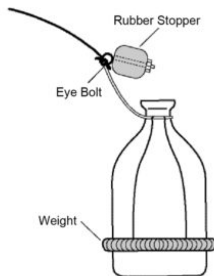
Fig. 3: A weighted-bottle sampler
