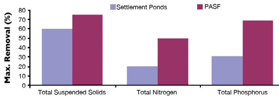
Fig. 1: Comparison of settlement pond and PASF wastewater treatment.
