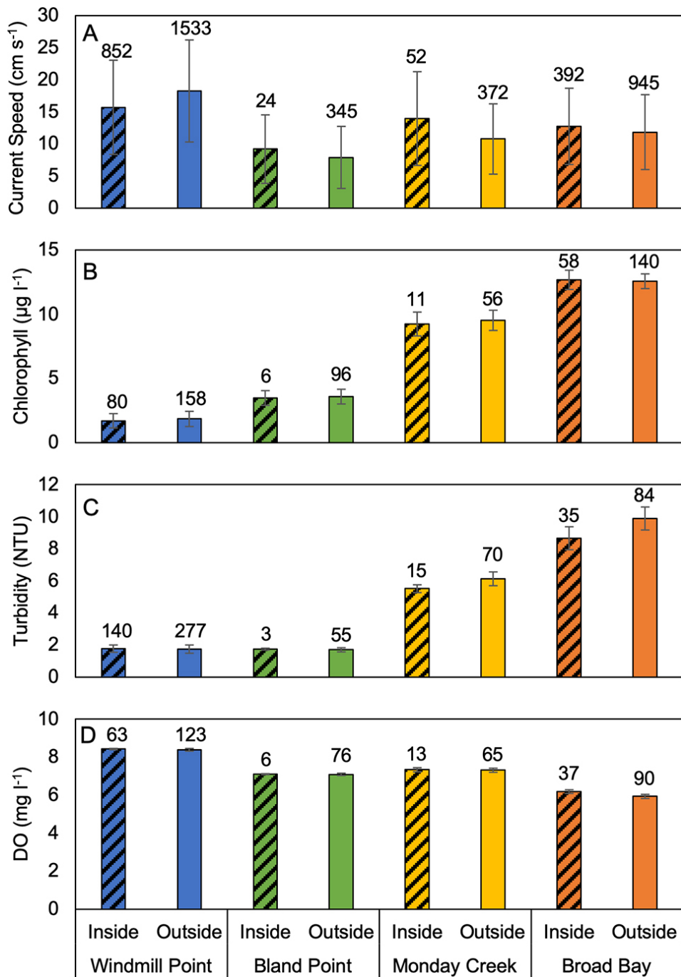
Fig. 1: Site comparison of current speed and water quality and during summer 2017. (A) Current speed, (B) chlorophyll, (C) turbidity and (D) DO. Error bars indicate \pm one standard deviation. Sample sizes are shown above each bar. Note that for sites with large sample sizes, \alpha = 0.05 confidence bounds on the means (not shown) are much smaller than the standard deviations.
