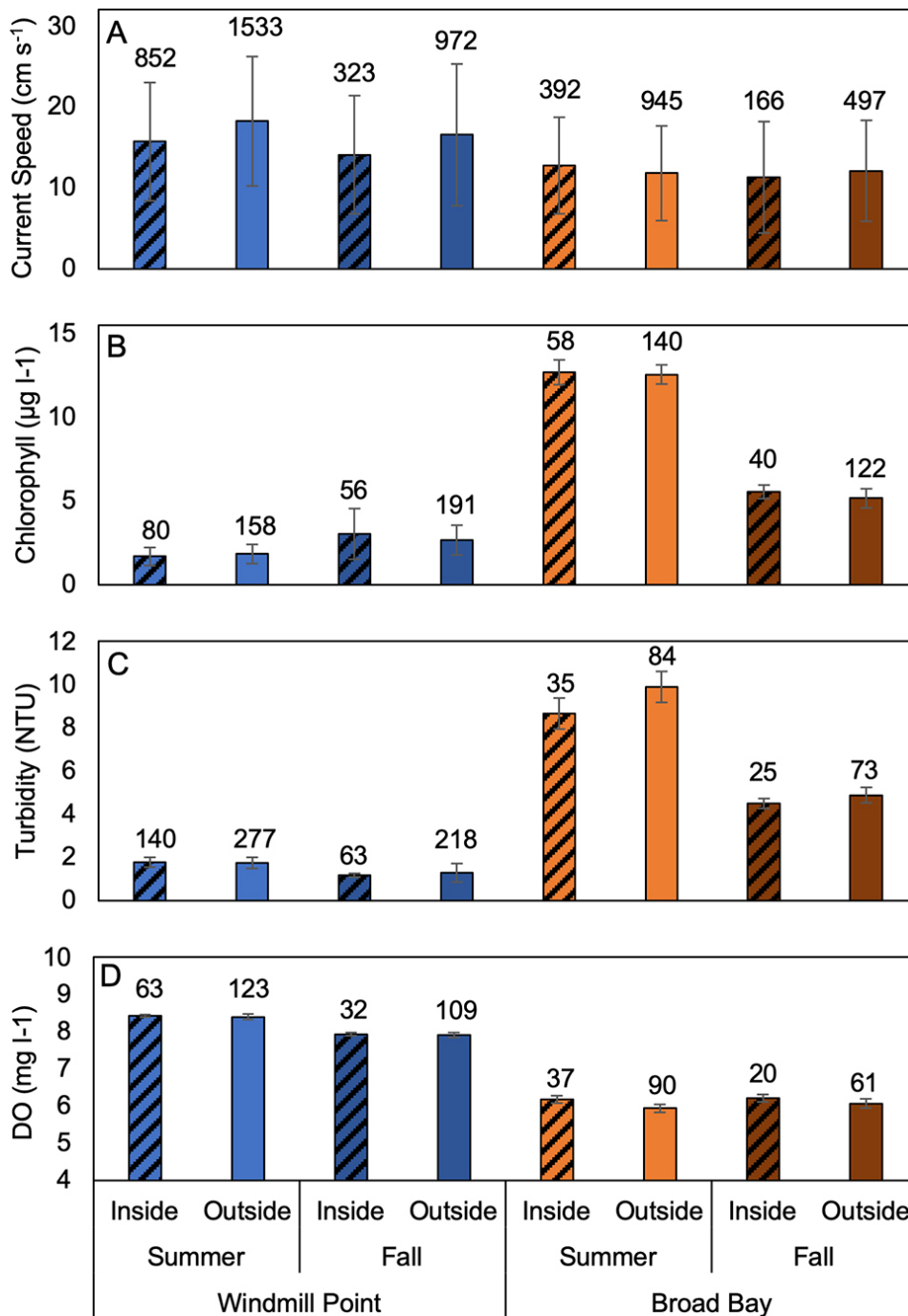
Fig. 2: Seasonal comparison of current speed and water quality at two sites. (A) Current speed, (B) chlorophyll, (C) turbidity and (D) DO. Error bars indicate \pm one standard deviation. Sample sizes are shown above each bar.
