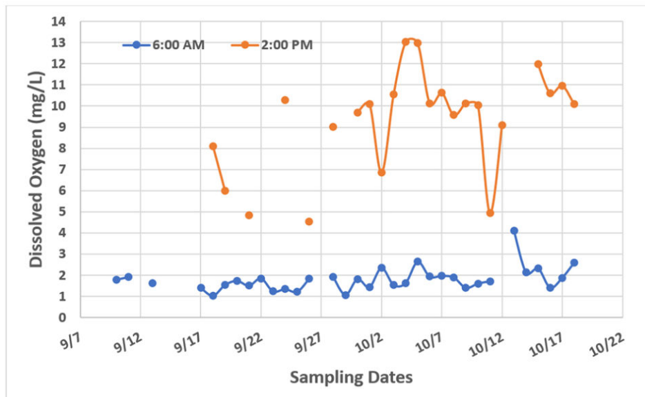
Fig. 2: Dissolved oxygen readings from inside raceway 2 at 6 a.m. and 2 p.m. during the IPRS trial.
